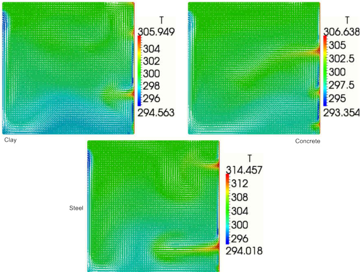
Figure 5.2: Temperature contours and velocity vectors after 2.5 hours
