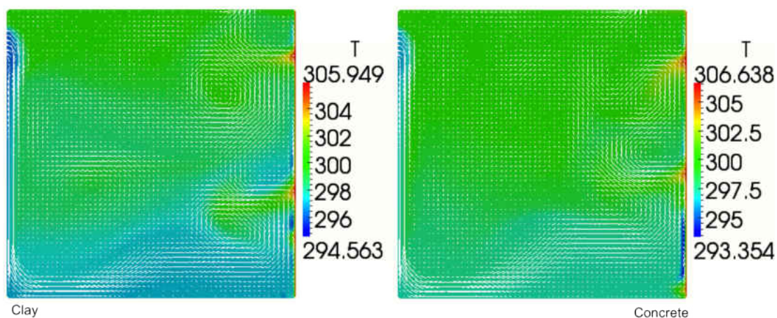
Figure 5.3: Temperature contours and velocity vectors after 3.75 hours
